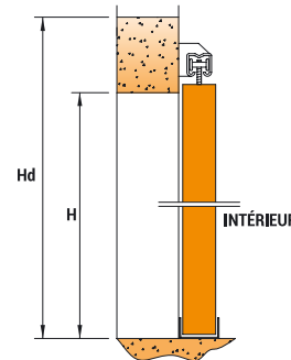
SECTIONS VERTICALE
