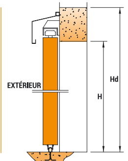
SECTIONS VERTICALE
